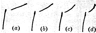
FIG. 8-20.—Steady-state characteristics showing from (a) to (d) the effect of decreasing heater power. A 500- \mu f condenser was connected in parallel to eliminate misfiring.
